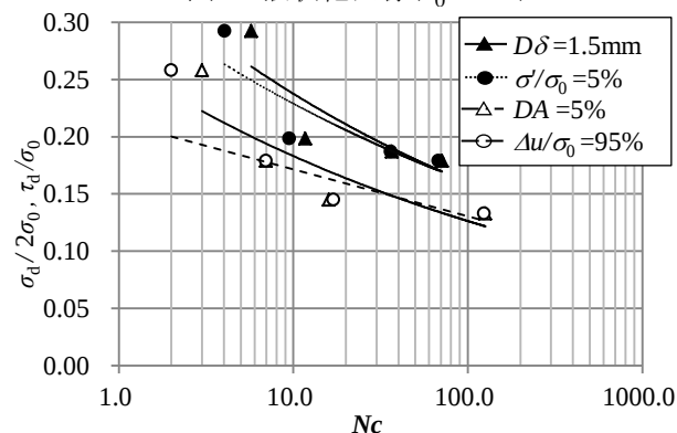
図3 液状化曲線( e_0=0.75 )
