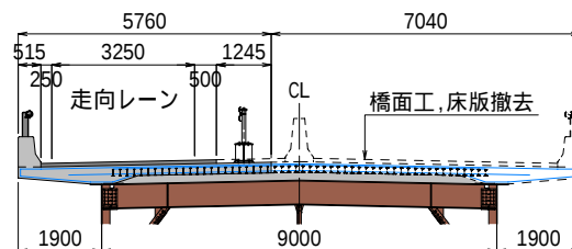
(a) 床版撤去-1
