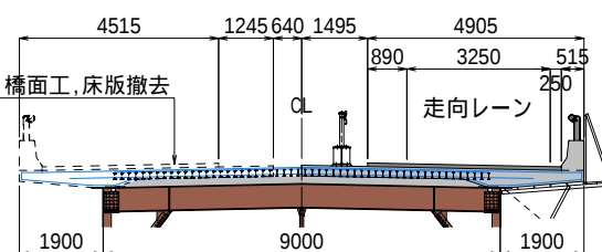
(c) 床版撤去-2
