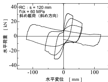
(a) RC 柱
