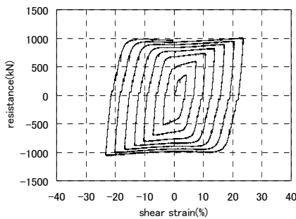
図6 変位漸増試験 (L100-24)
