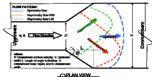
Fig. 1 Sudden Enlargement Open Channel
