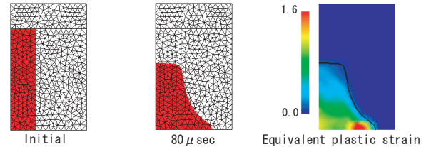
図-6 Present - Mesh1 (粗密なし)
