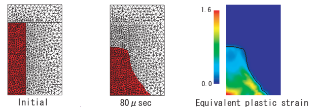
図-7 Present - Mesh2 (粗密あり)
