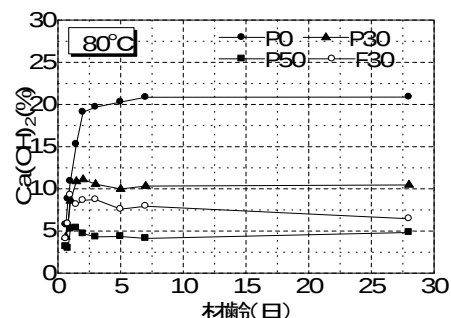
図-7 \text{Ca}(\text{OH})_2 量の経時変化 (80℃養生)
