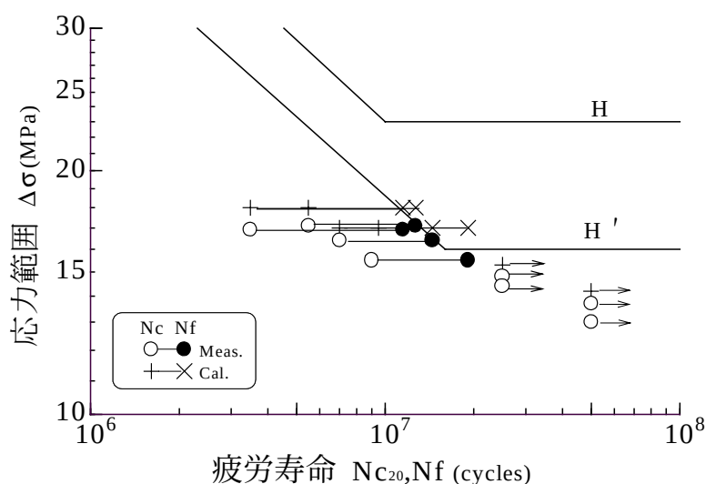
図-4 応力範囲と疲労寿命の関係
