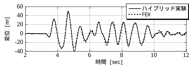
(c) X方向の変位応答
