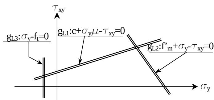
Figure 1. Linearised “cap model” for unreinforced masonry wall ( f_t : mortar adhesion, c : mortar shear strength, f'_m : block compression strength)
