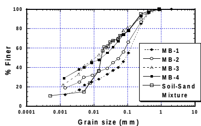
Figure 1. Grain size distributions of old adobe and soil-sand mixture used in this study.
