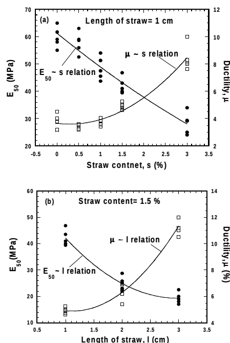
Figure 5. Relationships of (a) E_{50} \sim s and \mu \sim s , (b) E_{50} \sim \ell and \mu \sim \ell .
