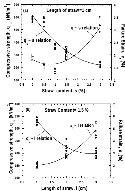
Figure 4. Relationships of (a) q_u \sim s and \epsilon_f \sim s , (b) q_u \sim \ell and \epsilon_f \sim \ell .
