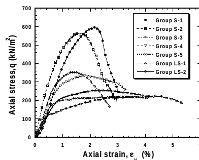
Figure 3. Typical stress-strain relationships of each group.
