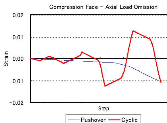
Fig. 7 Axial Load omission for cyclic and pushover
