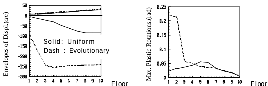
Figure 2 Displacements and Plastic Rotations at Joints of Columns and Beams
