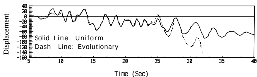
Figure 2 Displacement Response Histories at the Top Floor(cm)
