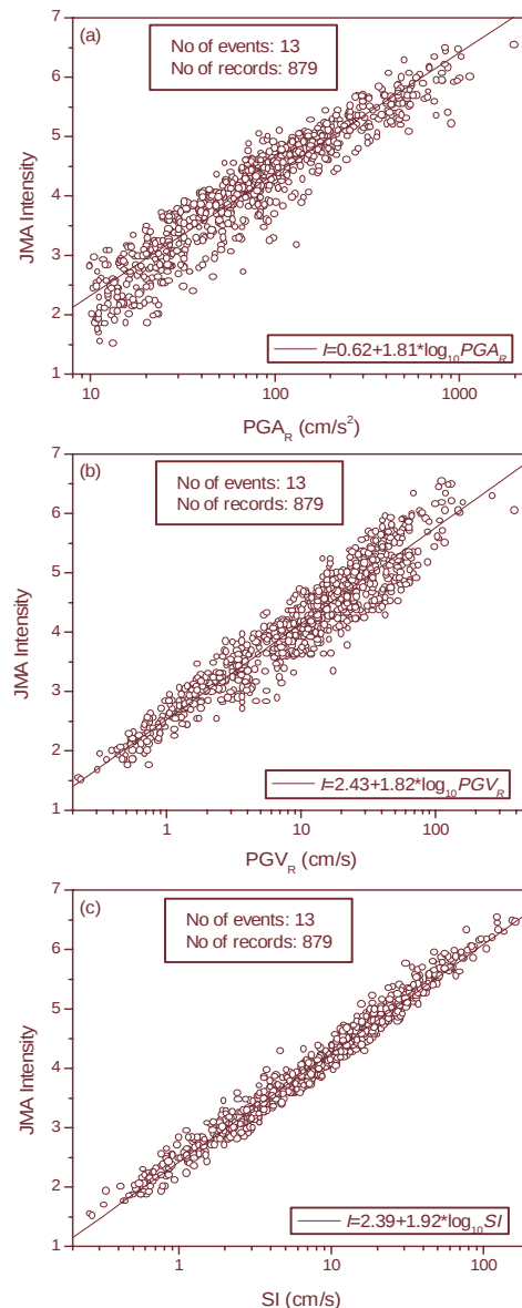
Fig. 1 Relationship between the JMA seismic intensity and ground motion indices
