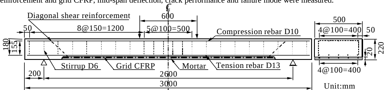
Fig.1 Detail of specimen
