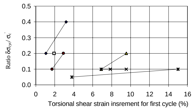
Fig. 6. Torsional shear strain increment after first cycle (lines does not represent the shear strain increment for the range between observed results)
