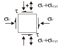
Fig. 3. Forces acting on the soil element
