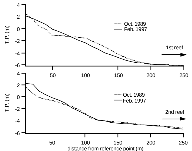
Figure 6 profile in the lee of reefs
