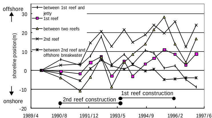
Figure 2 shoreline change
