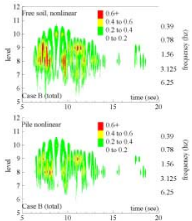
Fig. 6 Transient acceleration feature at interface level
