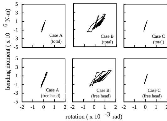
Fig. 3 Moment-rotation hysteresis of pile at G.L. -7 m
