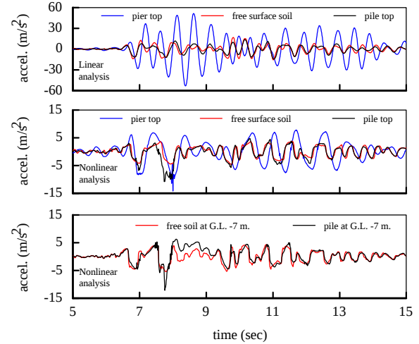
Fig. 5 Case B (total) acceleration time history
