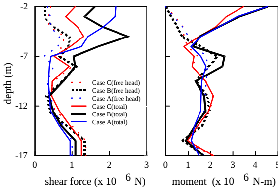
Fig. 2 Pile maximum internal forces
