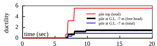
Fig. 7 Ductility at top of pile for Case
