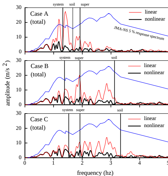
Fig. 4 Fourier amplitudes of pile top acceleration
