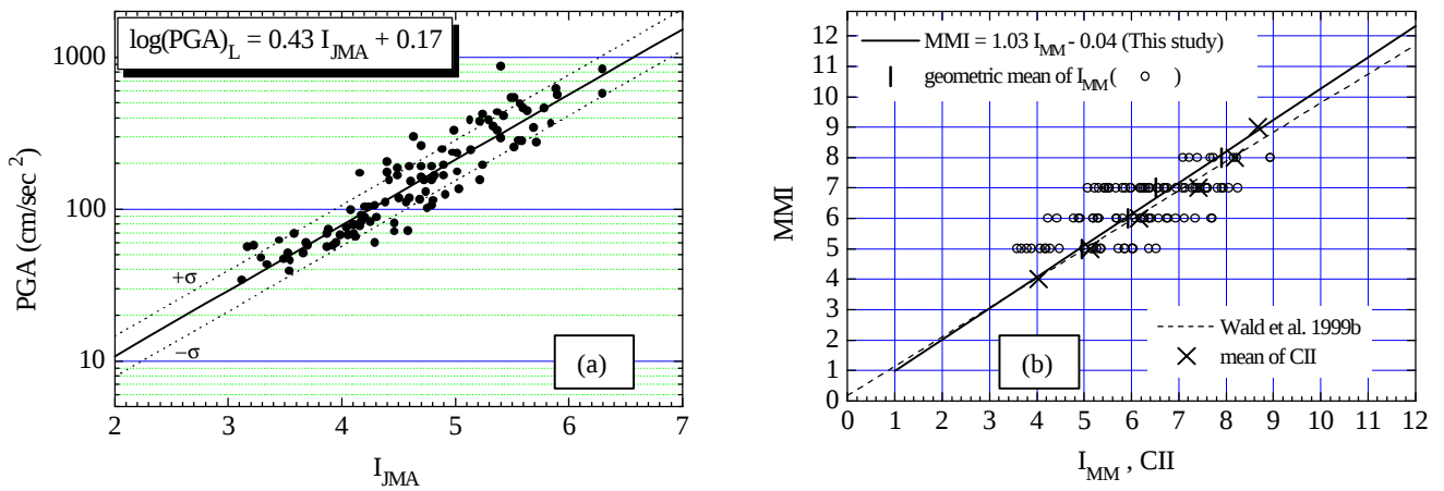
Fig. 2 The linear relations between (a) PGA and I_{JMA} and (b) MMI and I_{MM} (solid line) for the three California earthquakes.
