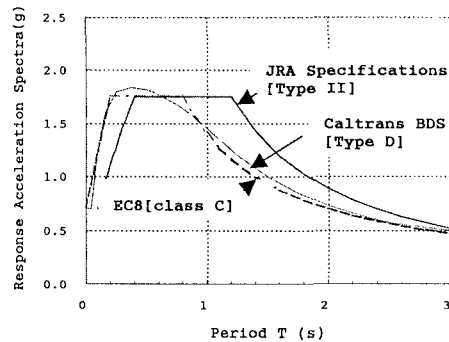
Fig. 2 Comparison of Response Acceleration Spectra among JRA, Caltrans and Eurocode 8
