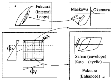
Fig. 2. Constitutive Relationships Used in Fiber Model
