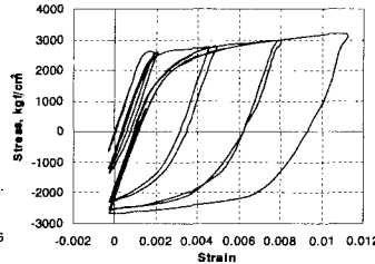
Fig. 5. Steel Stress Strain History
