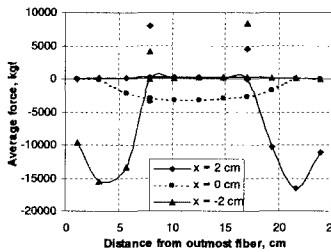
Fig. 7. Force Distribution in Fibers
