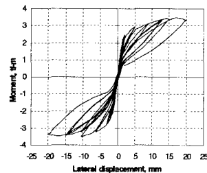
Fig. 9. Moment Carried by Concrete Fibers
