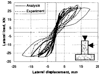
Fig. 4. Load-Displacement Relationship
