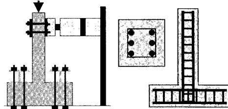
Fig. 1. Experimental Setup and Specimen
