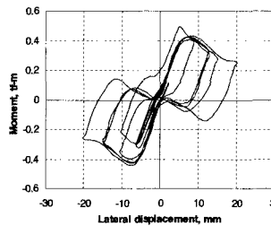
Fig. 8. Moment Carried by Steel Fibers
