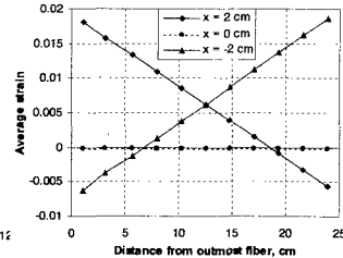
Fig. 6. Strain Distribution in Fibers
