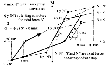
Fig. 2. RC hysteresis rule
