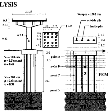
Fig. 1. Typical bridge pier and its model for analysis
