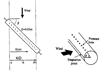
Fig.2-1 Cable model Fig.2-2 Position of Pressure hole
