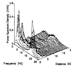
Fig.3-2 Power spectrum density of unsteady pressure on stationary cable model (with end plates, \beta=45^\circ , \theta=135^\circ , V=4\text{m/s} , in smooth flow)
