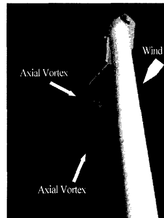
Photo.5-1 Flow visualization in a wake of inclined cable model (without end plates, \beta=45^\circ , V=0.5\text{m/s} , in smooth flow)
