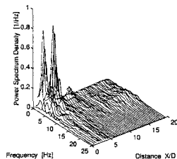
Fig.4-2 Power spectrum density of unsteady pressure on forced vibrating cable model (with end plates, \beta=45^\circ , \theta=135^\circ , V=4\text{m/s} , in smooth flow, \eta=0.01\text{m} , f=2\text{Hz} , V/fD=40 )
