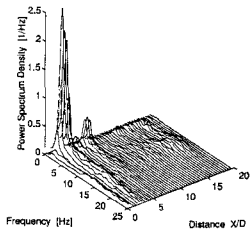
Fig.4-1 Power spectrum density of unsteady pressure on forced vibrating cable model (without end plates, \beta=45^\circ , \theta=135^\circ , V=4\text{m/s} , in smooth flow, \eta=0.01\text{m} , f=2\text{Hz} , V/fD=40 )
