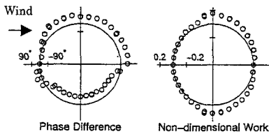
Fig.4-3 Distribution of phase difference \phi and non-dimensional work W_r around forced vibrating cable model ( X/D=2.56 , without end plates, \beta=45^\circ , V=4\text{m/s} , in smooth flow, \eta=0.01\text{m} , f=2\text{Hz} , V/fD=40 )
