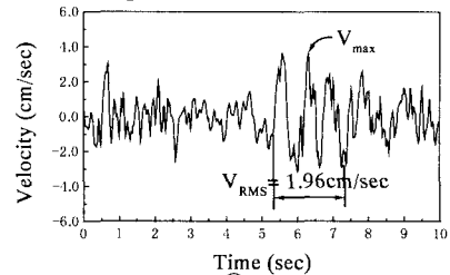
Measured point ② in Gerber girder bridge
