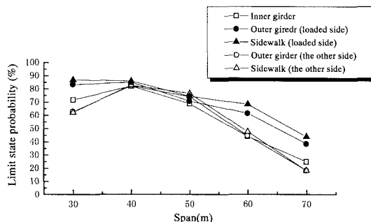
Fig.3 Limit state probability (vehicle speed 10m/sec)
