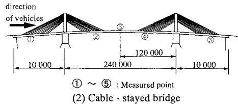
Fig.1 Points of measurement
