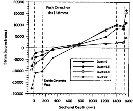
Fig. 3 (b) Longitudinal Strain Profiles (HF2)
