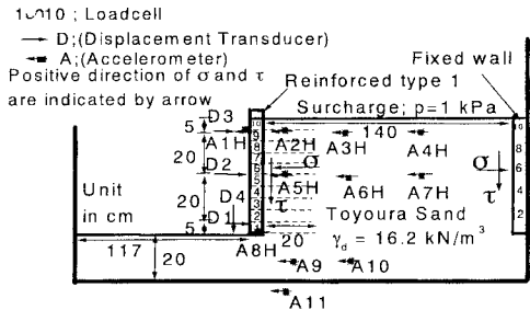
Fig. 1 Cross section of model test for reinforced type 1 and fixed wall type
