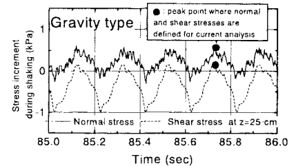
Fig. 6 Location of normal stress and shear stress used in analysis
