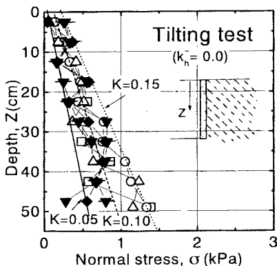
Fig. 2 Measured normal stress at initial condition for tilting test
