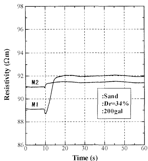
Fig.2 Resistivity changes of saturated sand (Dr=34%) during vibration at 200gal.
