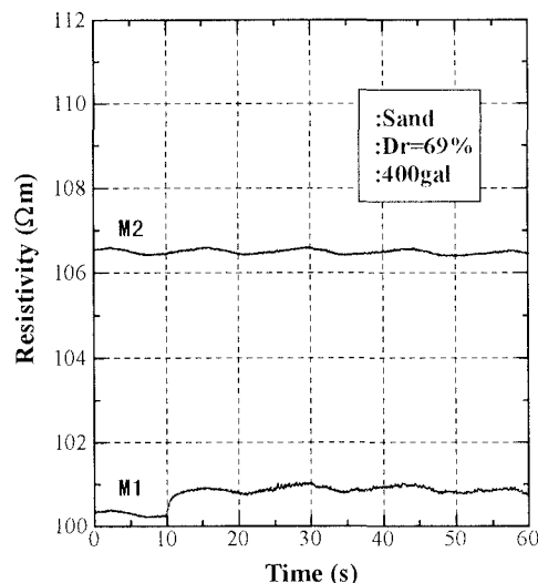
Fig.4 Resistivity changes of saturated sand (Dr=69%) during vibration at 400gal.
