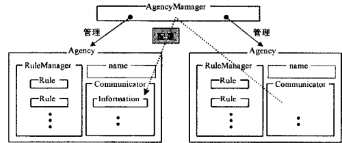
図2 AgencyManager, Agency, Ruleの構造
