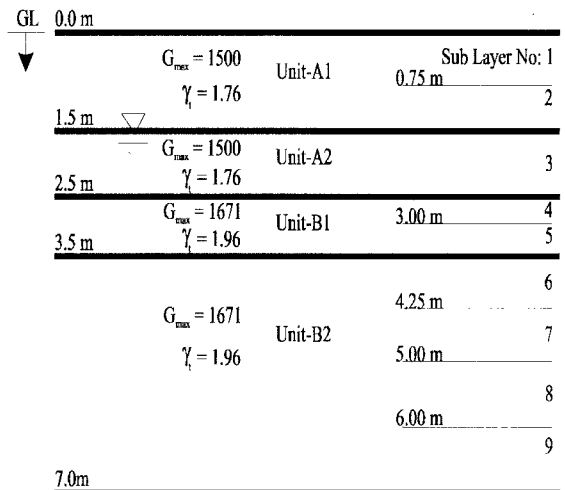
Fig. 3: Soil Condition and Layering
