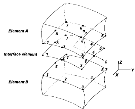
Fig. 1- Interface element
