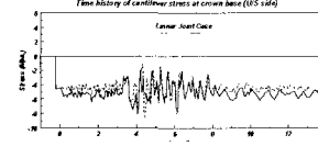
Fig. 10- Cantilever stress time history at the base of crown cantilever on U/S side
