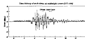
Fig. 8- Time history of arch stresses at midheight of crown cantilever on U/S face
