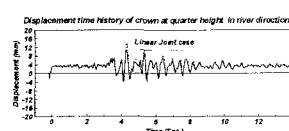
Fig. 6- Displacement time history in river direction at quarter height of crown cantilever
