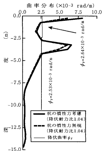
図-3 杭に生じる曲率分布 (Ⅱ種地盤)
