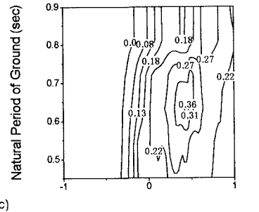
Fig.5 Response spectra in contour line
