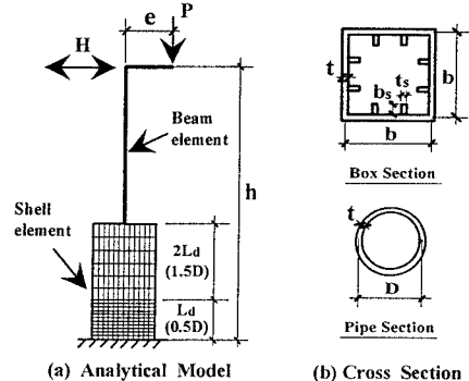
Fig. 1 Inverted L-shaped Columns
