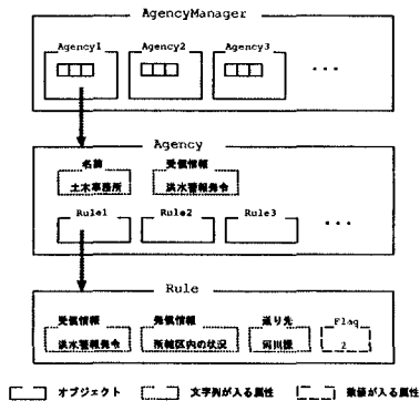
図2 AgencyManager, Agency, Ruleの構造
