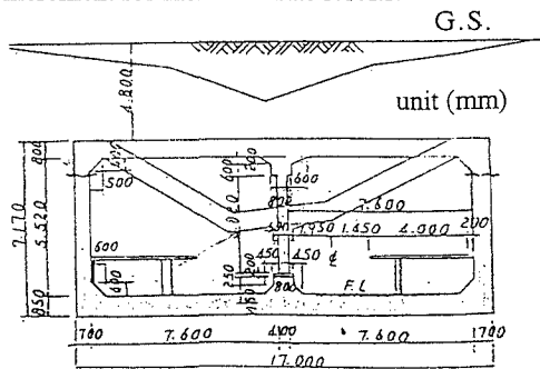
Fig.3a Tunnel failure shape
