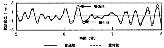
図-6 杭頭変位時刻歴波形 (SH-4)
