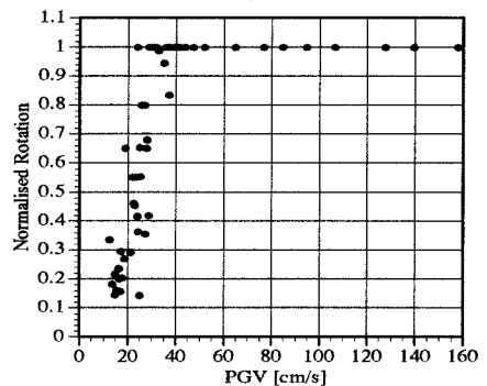
Figure 3. Normalised rotation versus PGV values of a block of h/b=4 and h=60 cm in response to sixty earthquake waves, all of PGA=0.4g.
