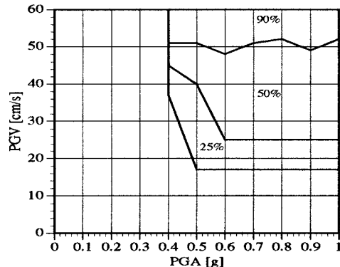
Figure 5. Probability of overturning of a block of h/b=3 and h=60 cm with respect to PGA and PGV.
