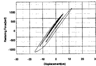
Fig.9 Hybrid Test for A3R(HN)
