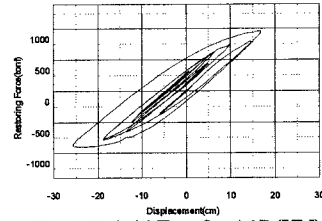
Fig.6 Hybrid Test for A1R(HN)
