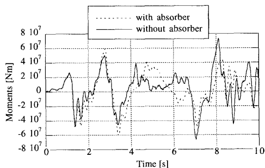
Fig.6 Moment histories for pier 9 with and without energy absorber
