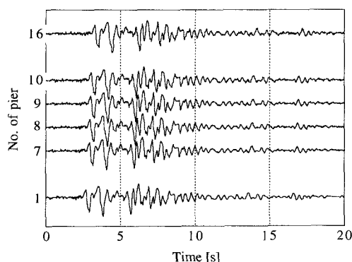
Fig.4 Simulated ground motions for Kobe Earthquake
