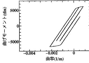
図-6-b 鋼製支承
