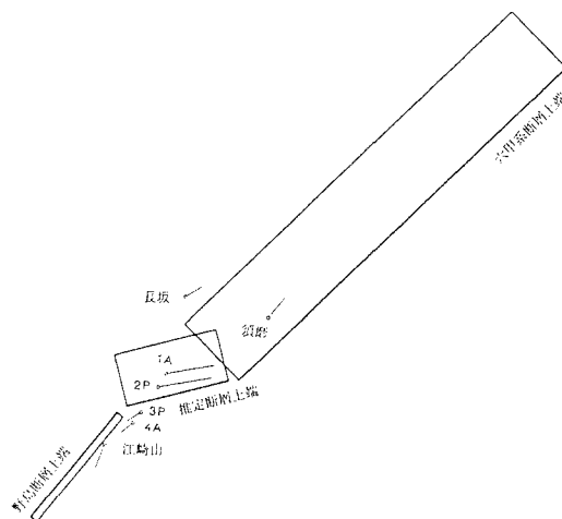
Fig. 4. Layout of fault planes and calculated displacements.
