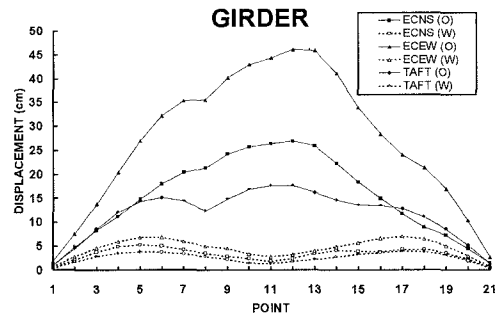
Fig. 6 Maximum Response
