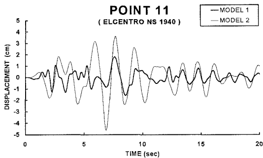
Fig. 7 Time History of Response
