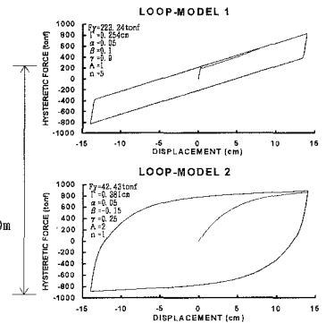
Fig. 2 Hysteresis Loop
