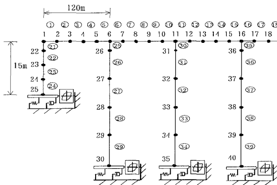
Fig. 1 Analysis Model
