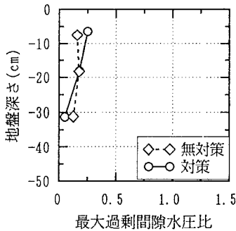
図-6 過剰間隙水圧比(sin50gal)
