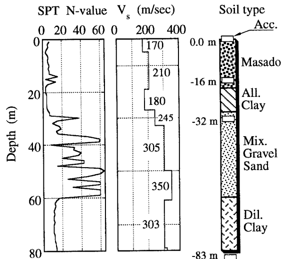
Fig. 1 Soil profile of the observation site at Port Island
