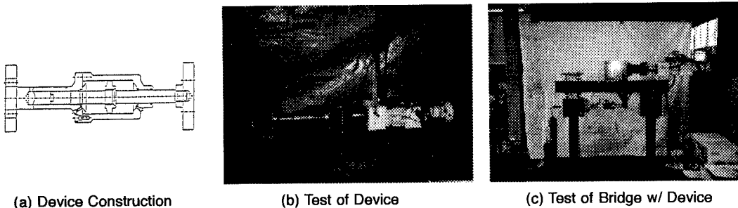
Fig. 1 Viscoelastic Device for Lateral Load Distribution
