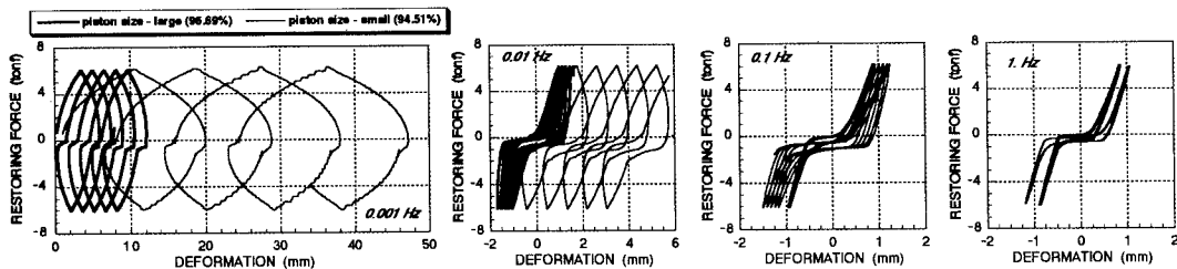
Fig. 2 Comparison of Load-Deformation Behavior of Device with Different Piston Sizes
