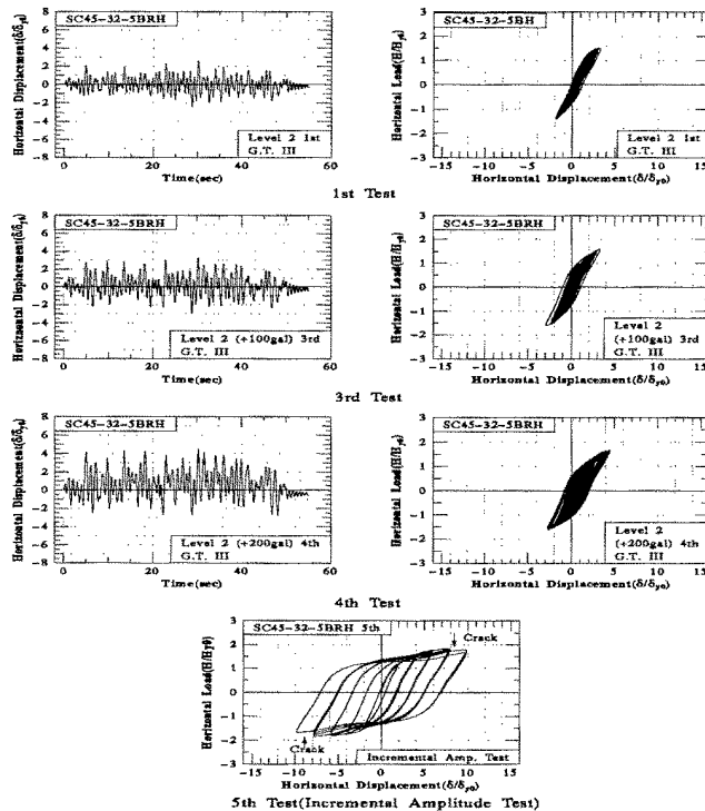
Fig.2 Response Curves(SC45-32-5BRH)
