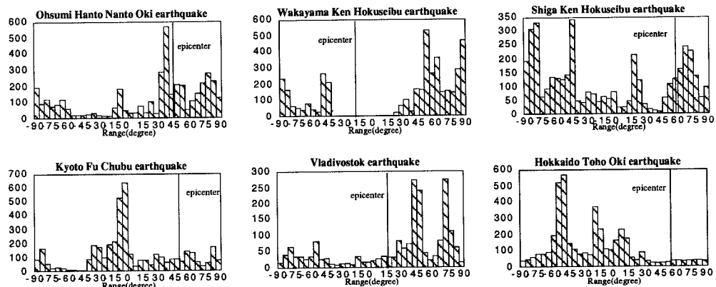
Fig.5 Strike Angle Histogram at site D.
