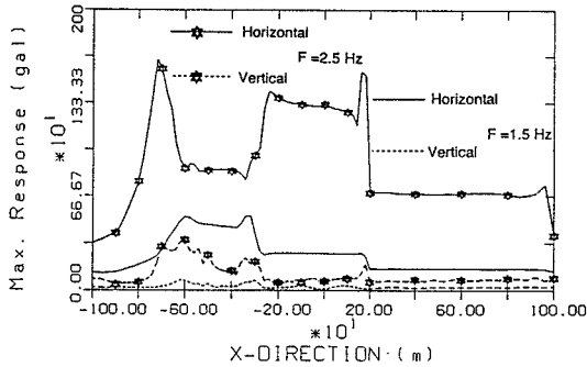
Fig. 2 Acceleration Response Comparison
