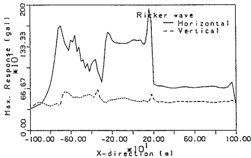
Fig. 5.a Max. Surface Acceleration
