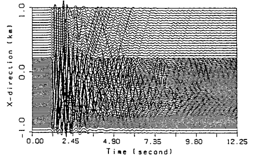
Fig. 5.b Hl. Acceleration Time History
