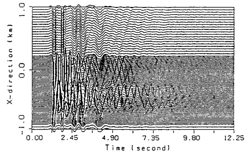
Fig. 4.b Hl. Displacement Time History
