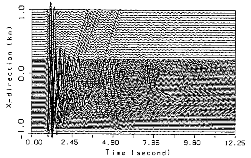
Fig. 3 Acceleration Time History (f=2.5 Hz)
