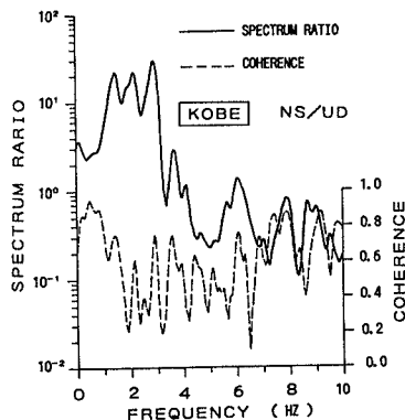
図-3 SPECTRUM RATIO
