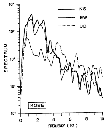
図-2 POWER SPECTRUM
