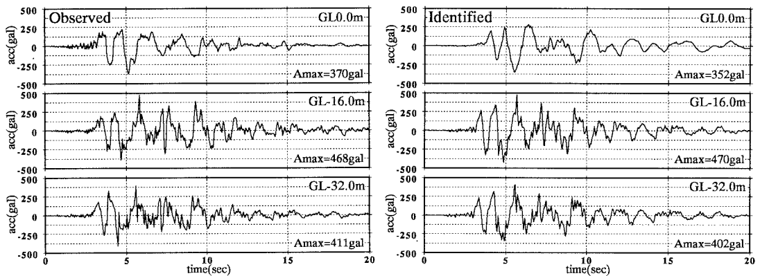
Fig.3 Comparison of waves between Observed and Identified
